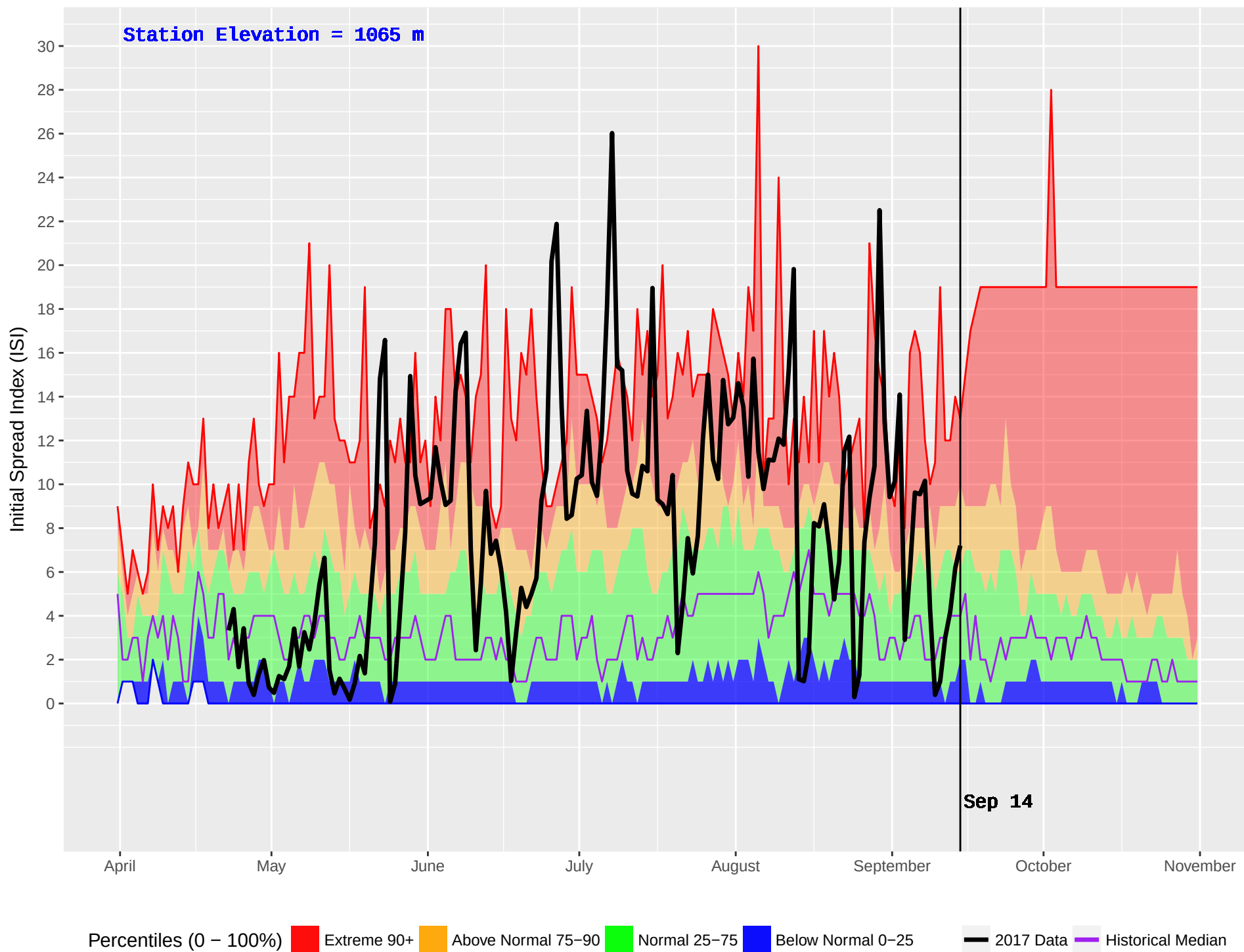
PLACE LAKE (212) : Historical (1981–2016) and Current (2017) Noon Initial Spread Index (ISI)
