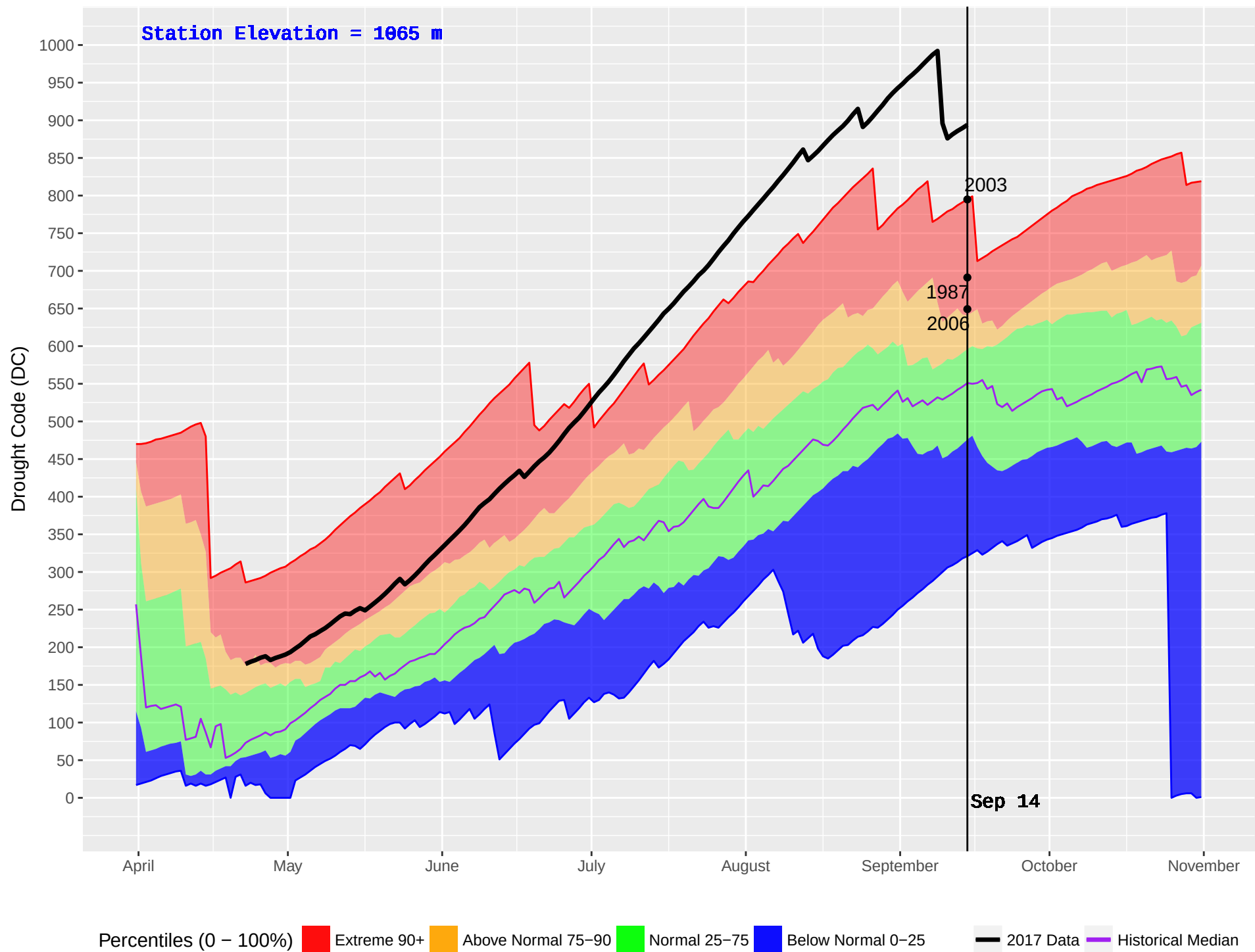
PLACE LAKE (212) : Historical (1981–2016) and Current (2017) Noon Drought Code (DC)
