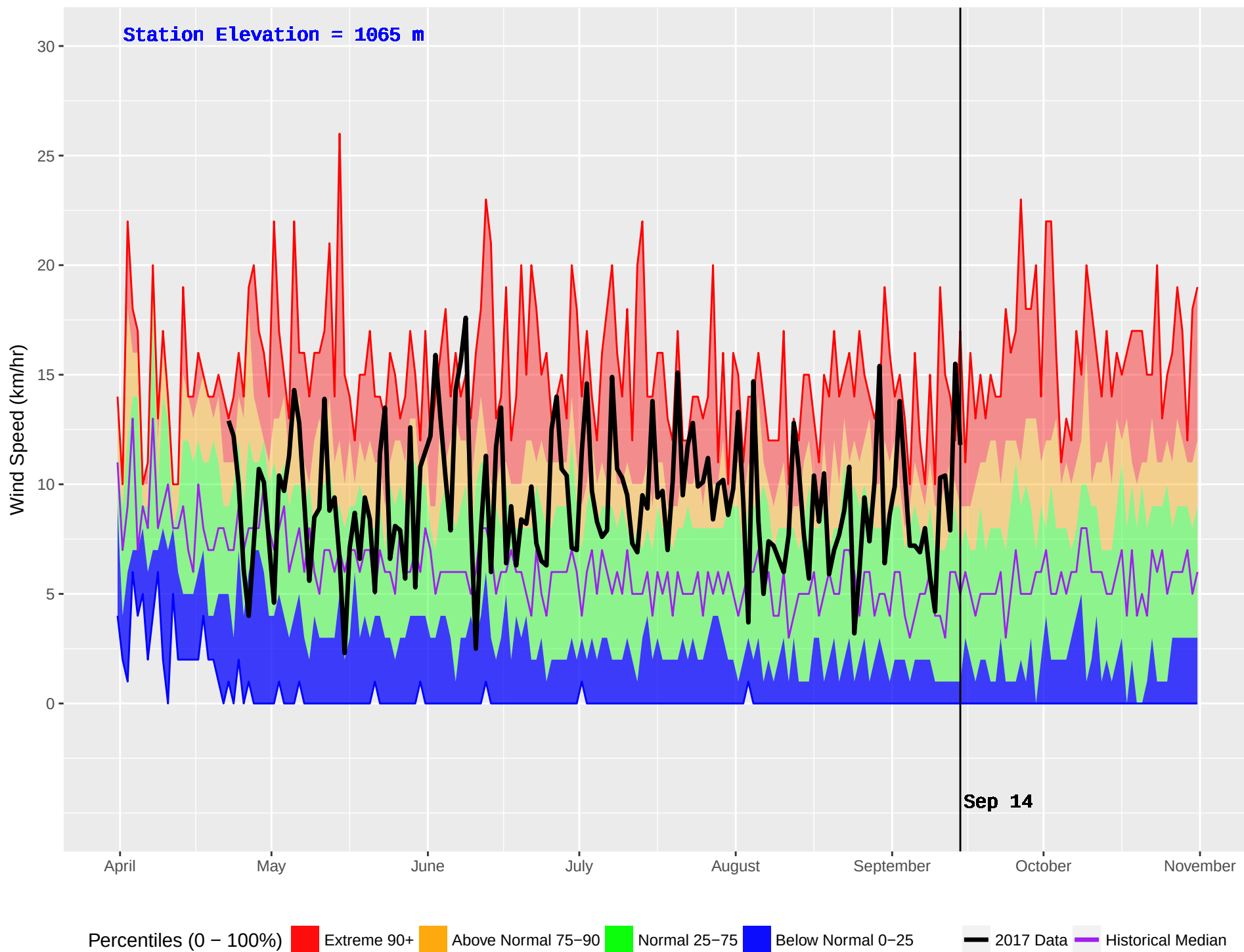
PLACE LAKE (212) : Historical (1981–2016) and Current (2017) Noon Wind Speed
