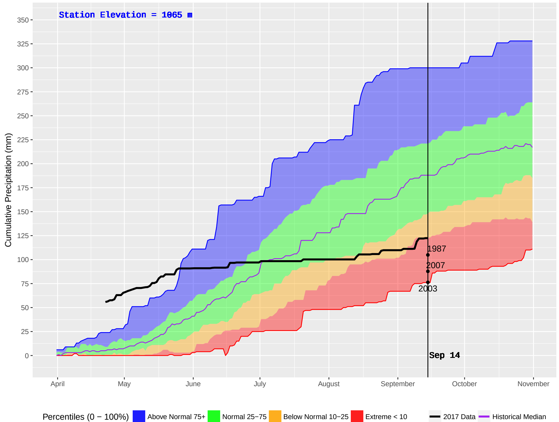
PLACE LAKE (212) : Historical (1981–2016) and Current (2017) Noon Cumulative Precipitation
