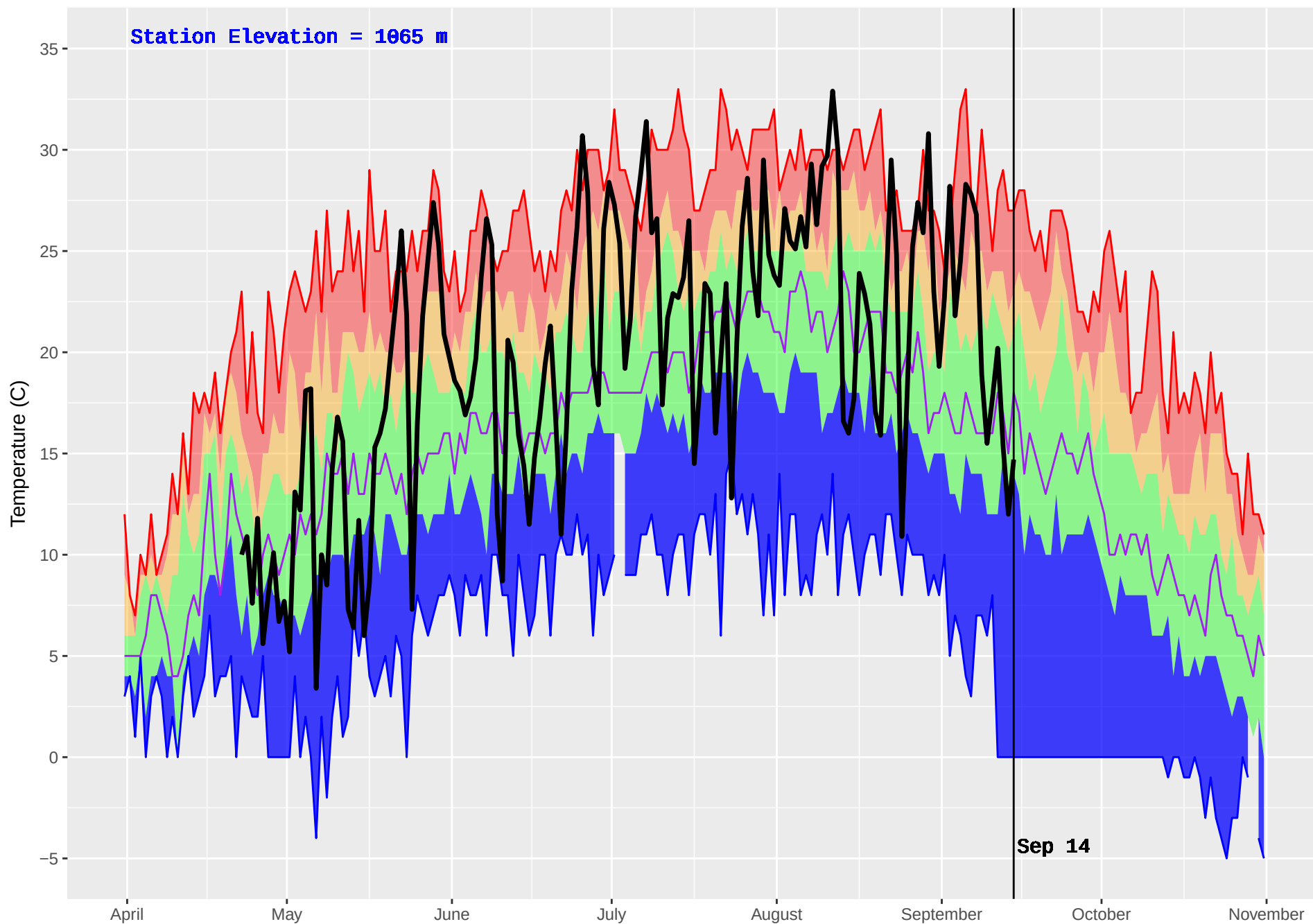
PLACE LAKE (212) : Historical (1981–2016) and Current (2017) Noon Temperature
