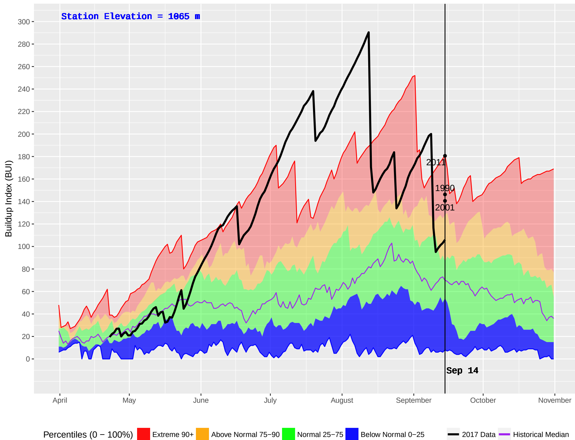
PLACE LAKE (212) : Historical (1981–2016) and Current (2017) Noon Buildup Index (BUI)
